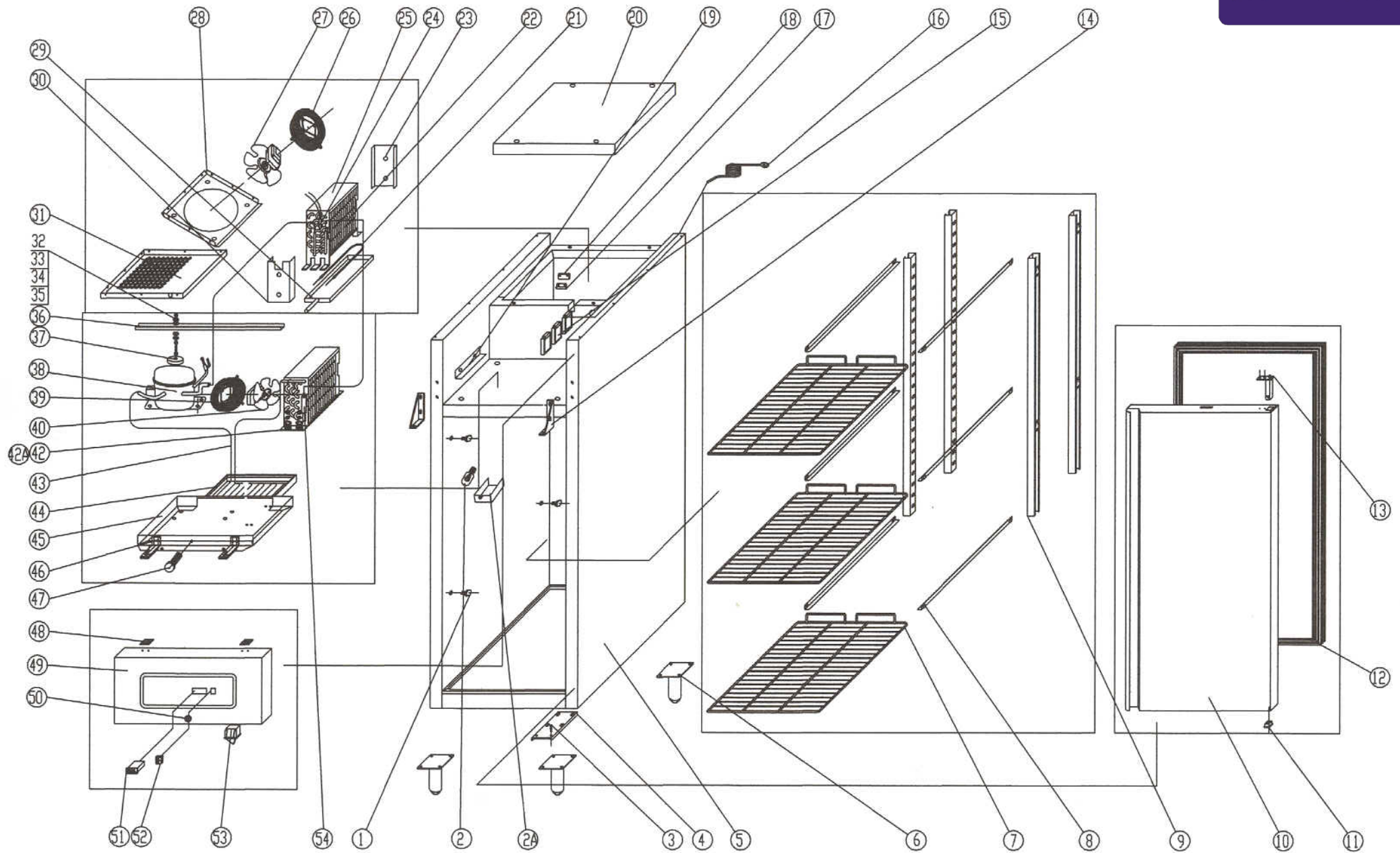
EXPLODE DIAGRAM OF RGN650BT
